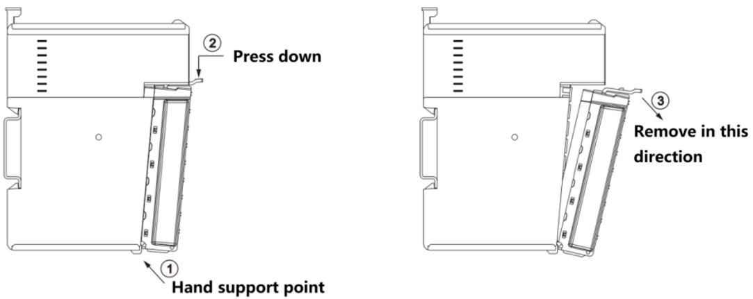
Fig.9.2-8 connector disassembly
