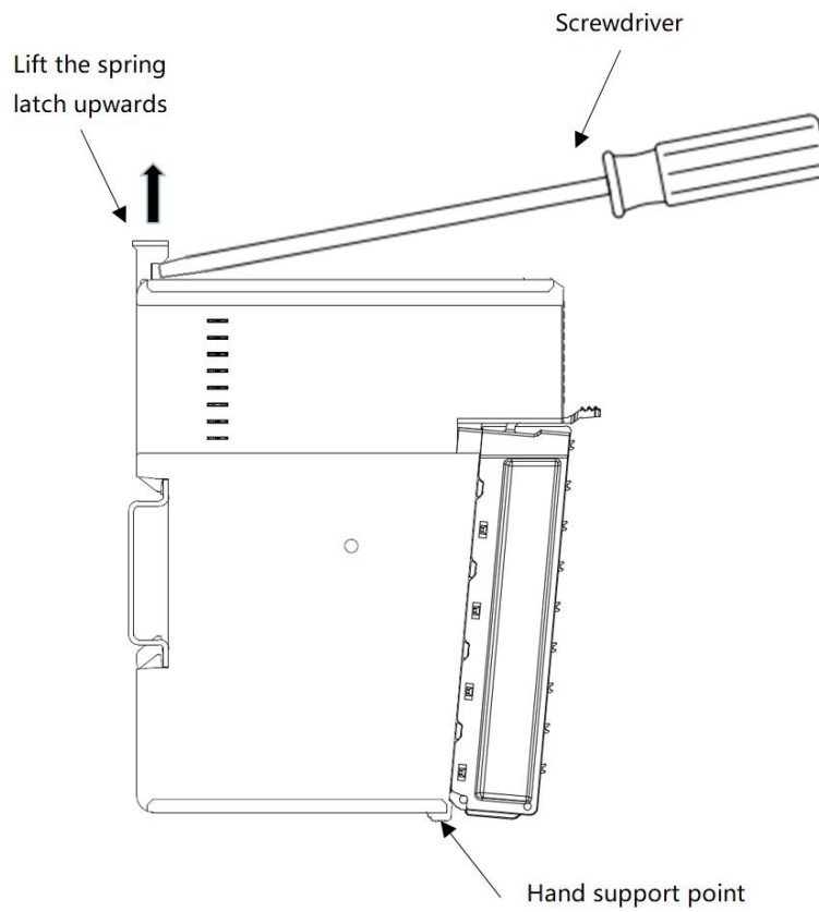
Fig.9.2-7 Module disassembly
