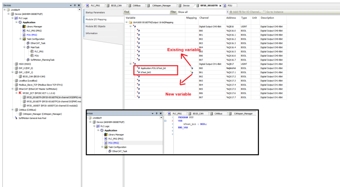
Fig. 10.2.1-9 Address mapping
