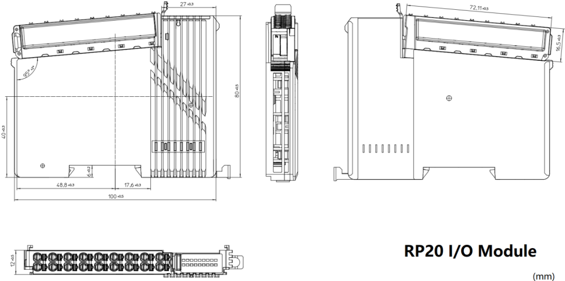
Fig.8.1-1 Dimensional drawing
