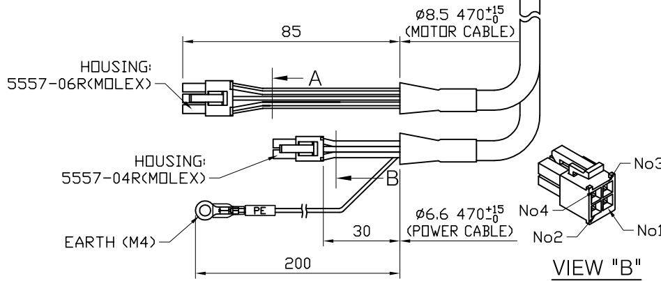
- PIN MAP (MOLEX 5557-04R)
