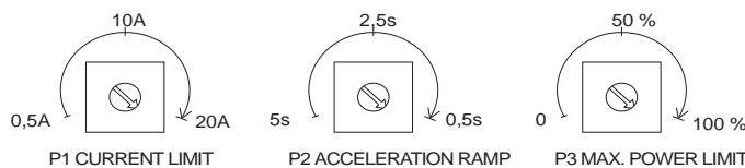
FIGURE 3. EM-12A ADJUSTMENTS.
